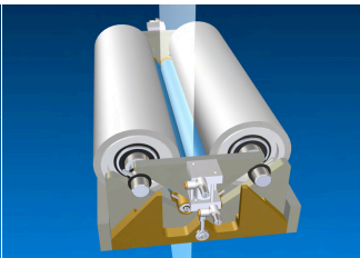
2 Roll Vertical Web Cleaner, 2 Sided Cleaning
